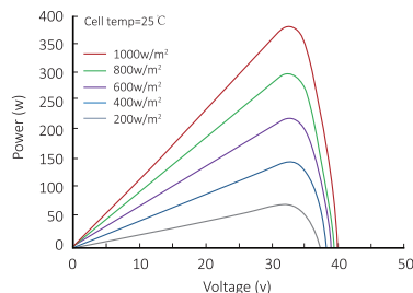
Power-Voltage Curve (LR4-60HIH-365M)
