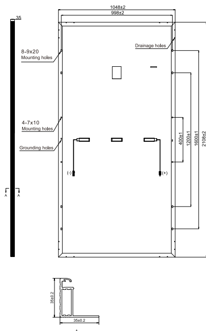
Dimensions of PV Module
